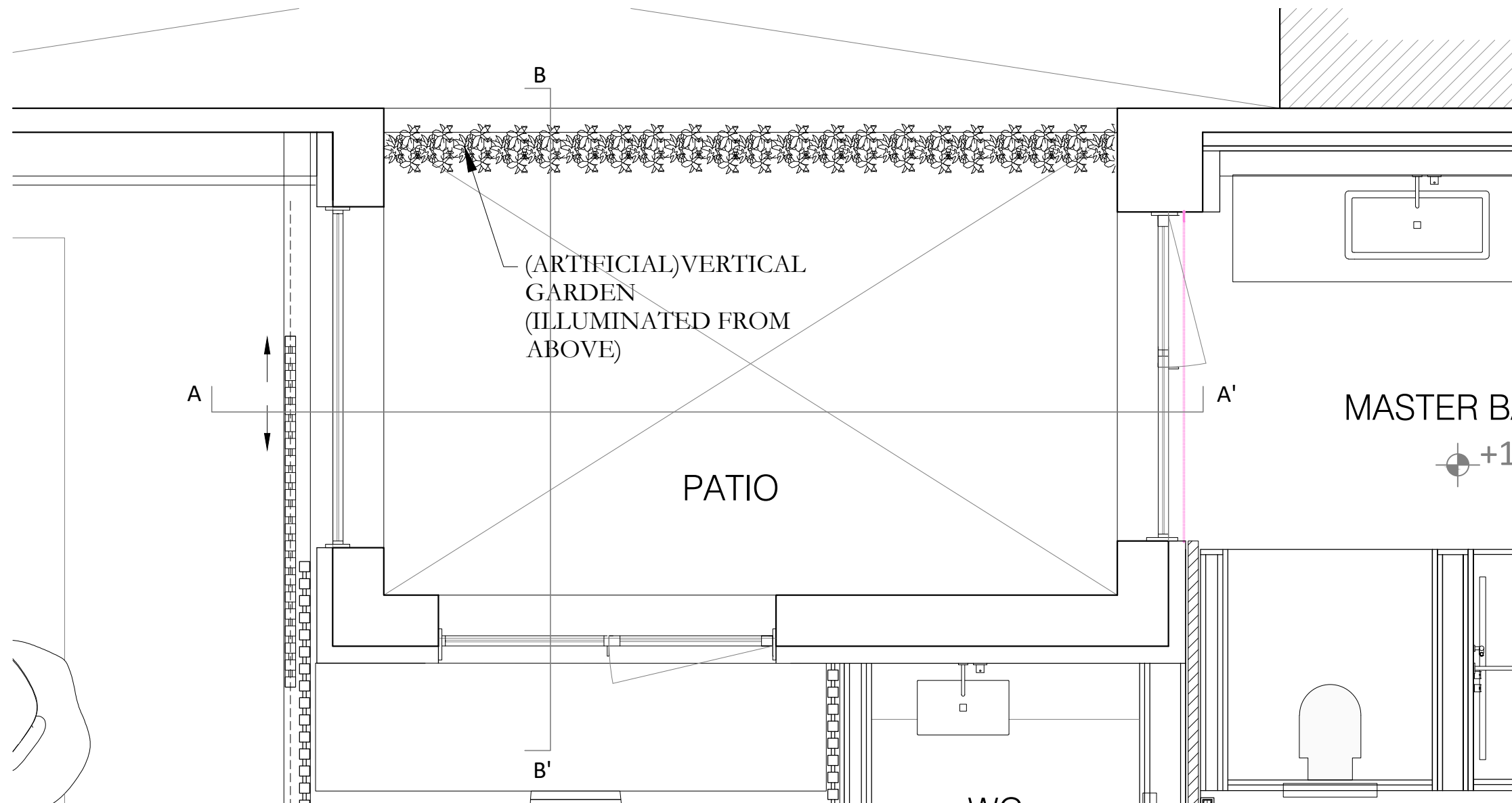
TOP VIEW VERTICAL GARDEN
