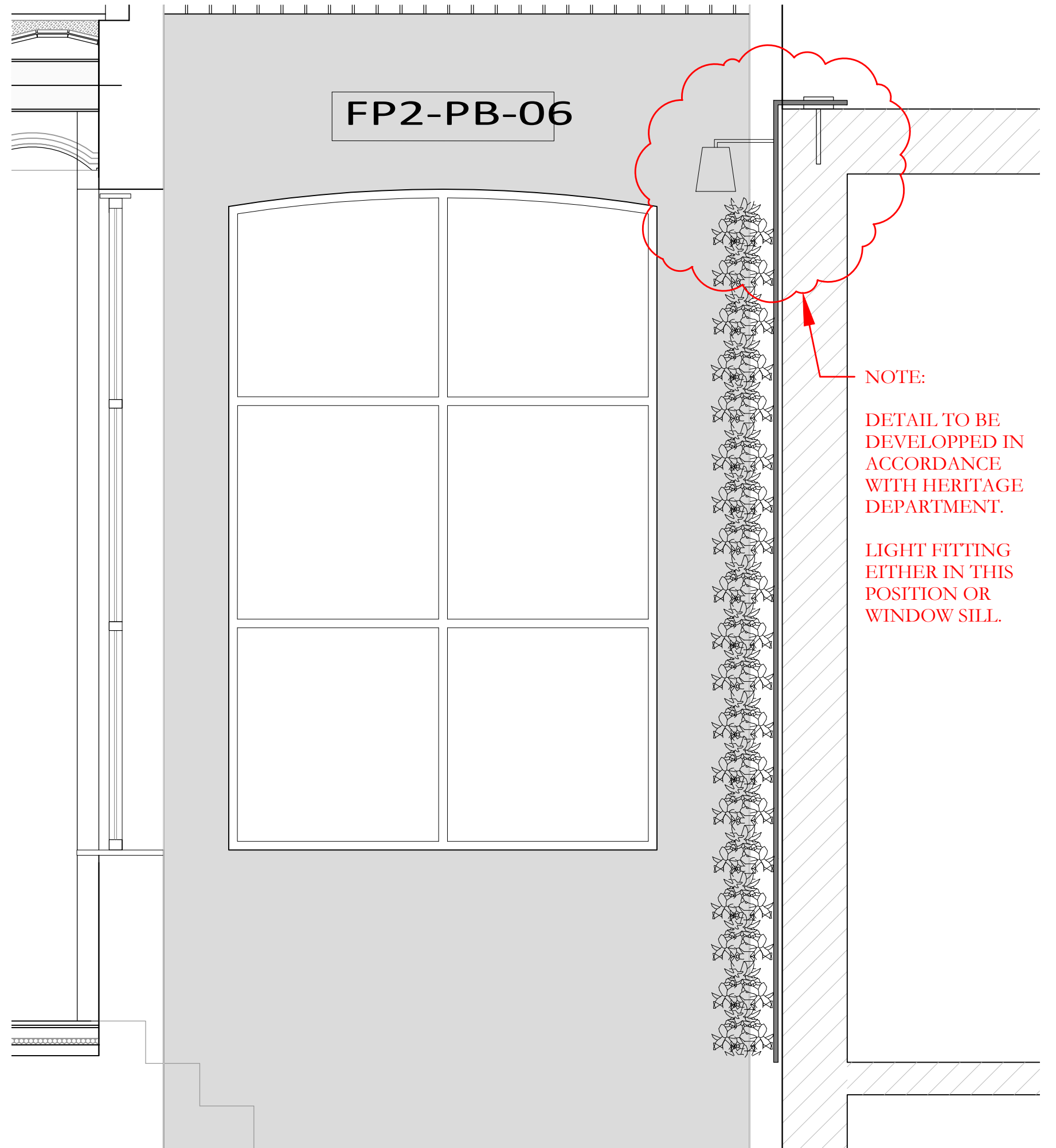
1:20 SECTION B VERTICAL GARDEN
