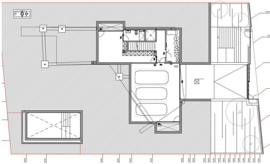
PLANTA SOTANO BASEMENT FLOOR
