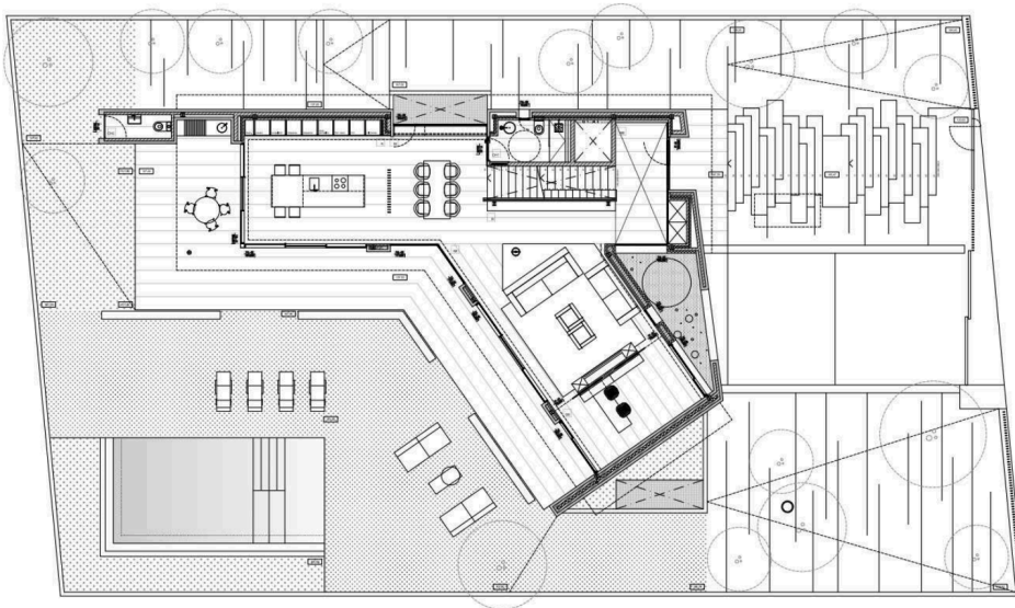
PLANTA BAJA GROUND FLOOR
